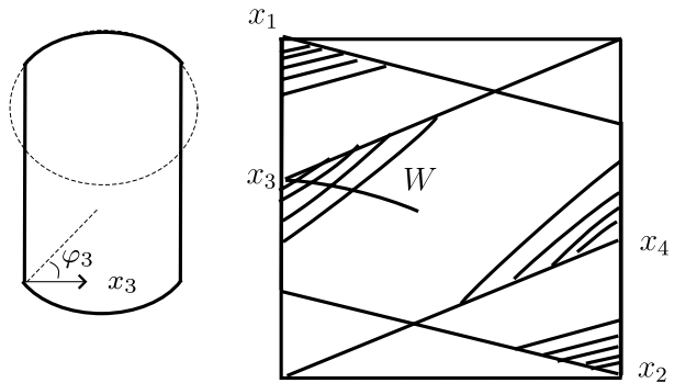
Fig. 1 Discontinuity manifolds of stadium
